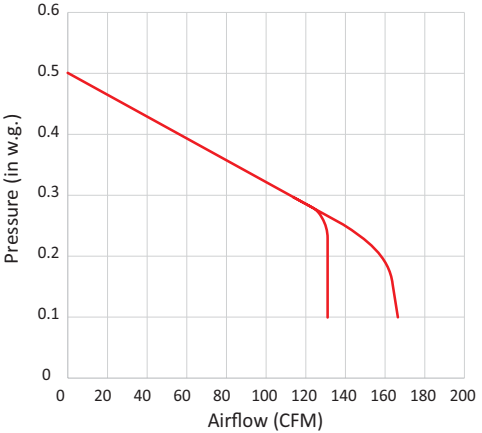
Fan curves with MERV 16 filter
