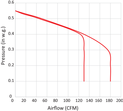
Fan curves with MERV 8 filter
