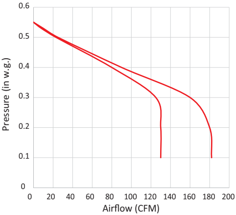
Fan curves with MERV 16 filter
